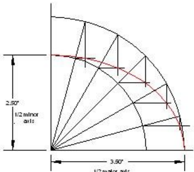
developing a quadrant of an ellipse
